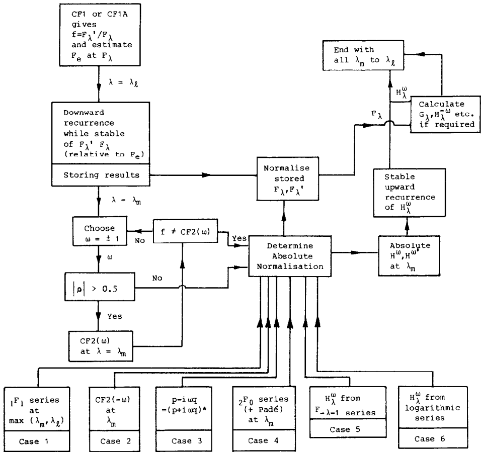
FIG. 3. Flow diagram for the evaluation of the complex Coulomb functions for the \lambda range \lambda_m to \lambda_l .
