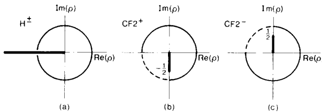
FIG. 1. Analytic ranges and cut positions of the logarithmic derivatives of H^\pm and the continued fractions CF2 + and CF2 - . In the dashed quadrants, CF2 ± do not equal the logarithmic derivatives of H^\pm .
